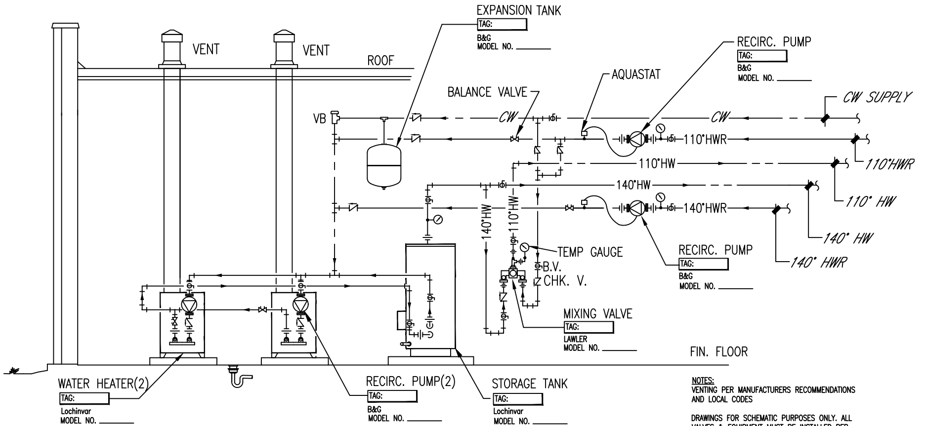
○ TWO CONDENSING HEATERS, ONE TANK, DUAL TEMPERATURE
